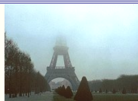
Stratus
